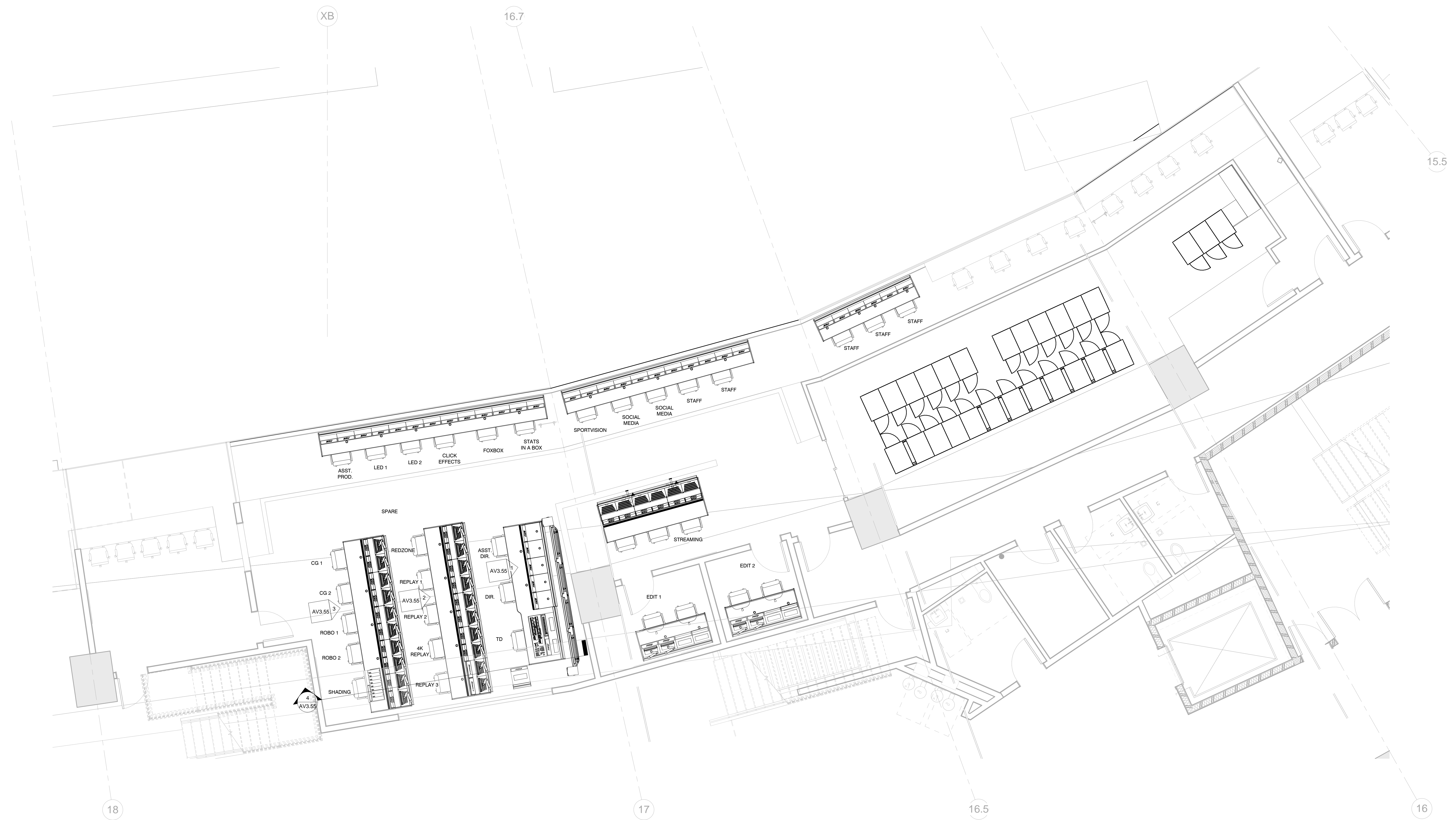
1 Production Control Room (PCR) Console Layout 1/4" = 1'-0"
