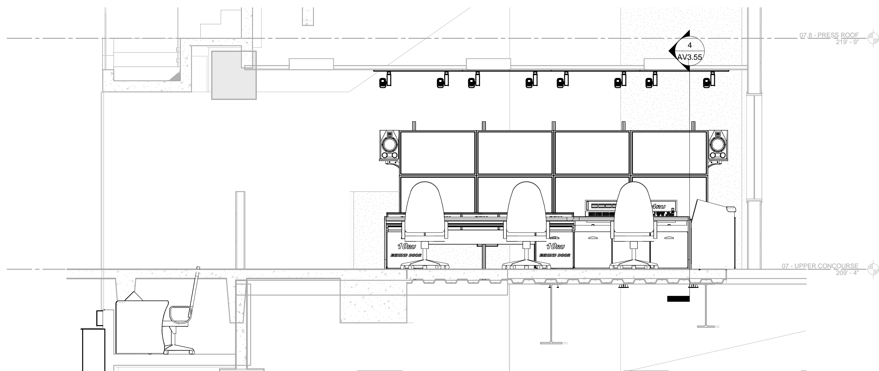
1 PCR Front Row Elevation 3/8" = 1'-0"
