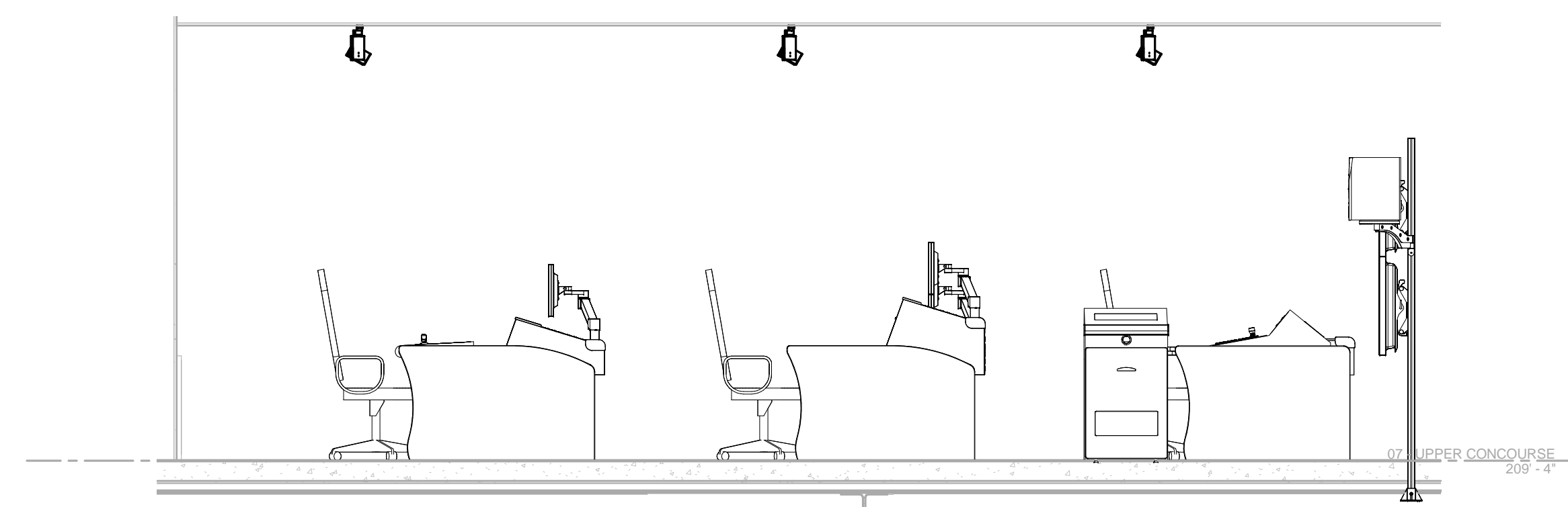
4 PCR Section 3/8" = 1'-0"
