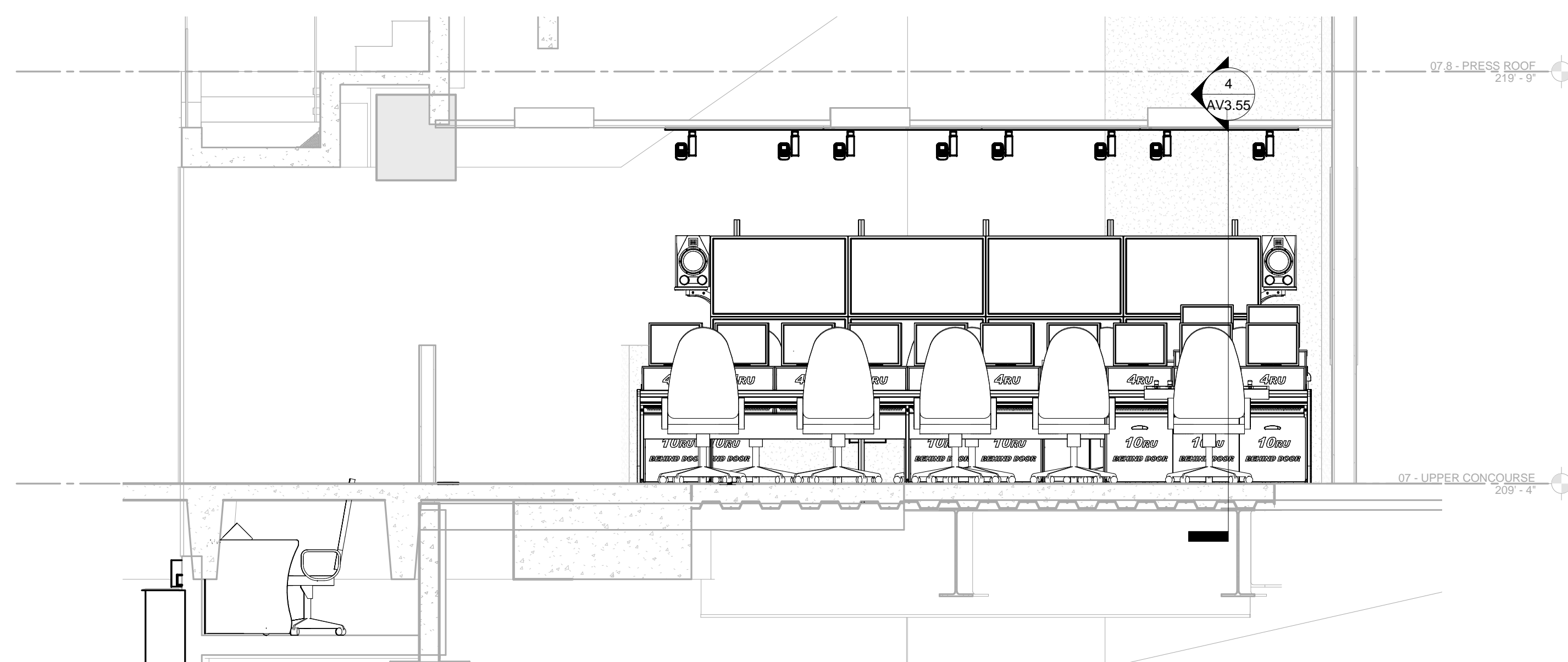
3 PCR Back Row Elevation 3/8" = 1'-0"
